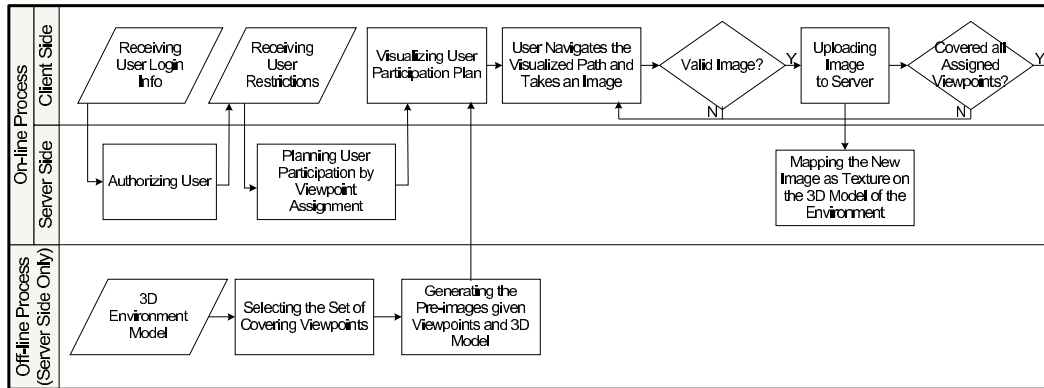
Figure 3: GeoSIM Workflow
