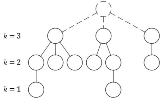
1 Search tree
